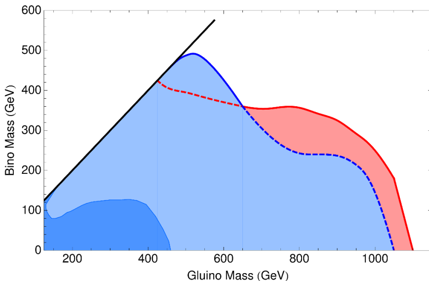
Figure 5. Discovery reach at the LHC for directly decaying gluino pair production at \mathcal{L} = 1 \text{ fb}^{-1} . In light blue, the reach of a high E_T set of searches, and the additional reach due to an \alpha_{\text{RTS}} search (red). Also shown is the 2\sigma exclusion at the Tevatron with 4 \text{ fb}^{-1} of data (dark blue) from [61].
