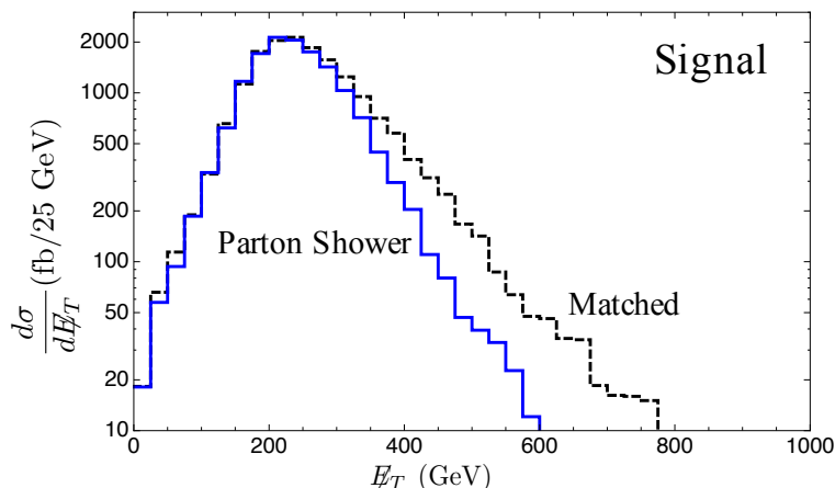
Figure 3. E_T distributions for a matched (black) and unmatched (blue) 250 GeV gluino decaying to a 200 GeV LSP.
