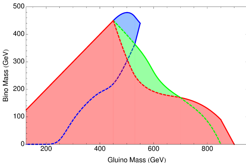
Figure 6. Discovery reach at the LHC for cascade-decaying gluino pair production at \mathcal{L} = 1 \text{ fb}^{-1} . In light blue, the reach of a high \cancel{E}_T \geq 600 \text{ GeV} set of searches, and the reach due to an \alpha_{\text{RTS}} search (red). The reach of a Base Search \cancel{E}_T \geq 400 \text{ GeV} is shown in green.
