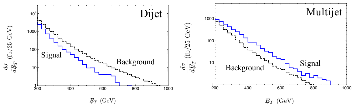
Figure 7. \cancel{E}_T distributions for SM backgrounds (black) and a 250 \text{ GeV } \tilde{q} (blue) decaying to a 50 \text{ GeV} LSP and a light flavored quark in dijet (left panel) and multijet (right panel) channels.
