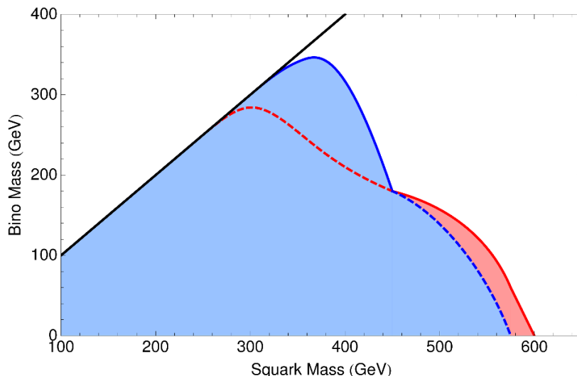
Figure 8. Discovery reach at the LHC with \sqrt{s} = 14 TeV and 1 \text{ fb}^{-1} . The light blue region shows the reach of the multijet and \cancel{E}_T high \cancel{E}_T search, and the reach of the \alpha_{\text{RTS}} is shown in dashed red.
