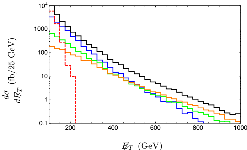
Figure 4. E_T distributions for t\bar{t} (blue), W^\pm (green), Z^0 (orange), QCD (dashed red) and combined (black) in the multi-jet channel, after applying the selection criteria.
