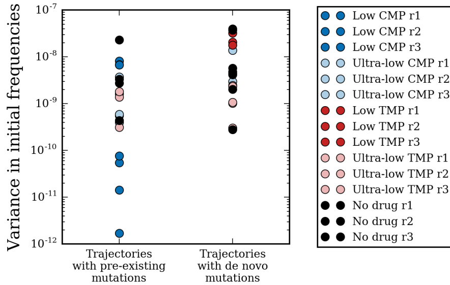
Supplementary Figure 15: Comparison of initial frequencies of trajectories in different types of clusters. For each trajectory cluster classified as having pre-existing or de novo beneficial mutations ( Supplementary Fig. 13 ), we calculated the variance of initial frequencies of trajectories in that cluster.
