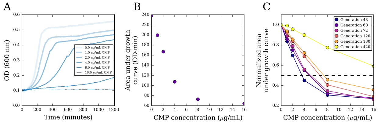
Supplementary Figure 4: Example of IC 50 calculation. (A) Growth curves of cells from a barcoded population evolving in low chloramphenicol (CMP) at generation 48 (passage 8), measured with different concentrations of CMP. (B) For each growth curve in (A), we calculated the area under it and plotted the area as a function of CMP concentration. (C) We similarly calculated growth curve areas for generations 48, 60, 72, 180, and 420 and normalized each by the area of the growth curve with zero CMP at the same time point. The IC 50 is then defined as the antibiotic concentration leading to 50% of growth relative to growth at zero CMP.
