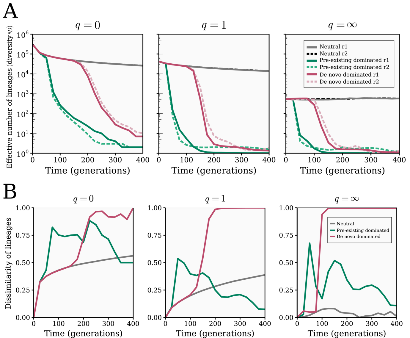
Extended Data Fig. 10 | Simulated dynamics of lineage diversity. We simulated evolutionary dynamics of the barcoded population for two replicates of each condition: “neutral” (no mutations), “pre-existing dominated,” and “de novo dominated” (see Methods). (A) For each population, we calculated the effective number of barcoded lineages using the diversity index {}^qD (Eq. 1; see also Methods) for three different values of q , which controls the weight of low- versus high-frequency lineages: {}^0D (number of unique barcodes, left), {}^1D (Shannon diversity, center), and {}^\infty D (reciprocal of the maximum lineage frequency, right). (B) We also calculated the dissimilarity of lineages (Eq. 2; see also Methods) among all replicate populations in each condition, using q=0 (left), q=1 (center), and q=\infty (right). All diversity and dissimilarity values are based on perfect sampling of the population.
