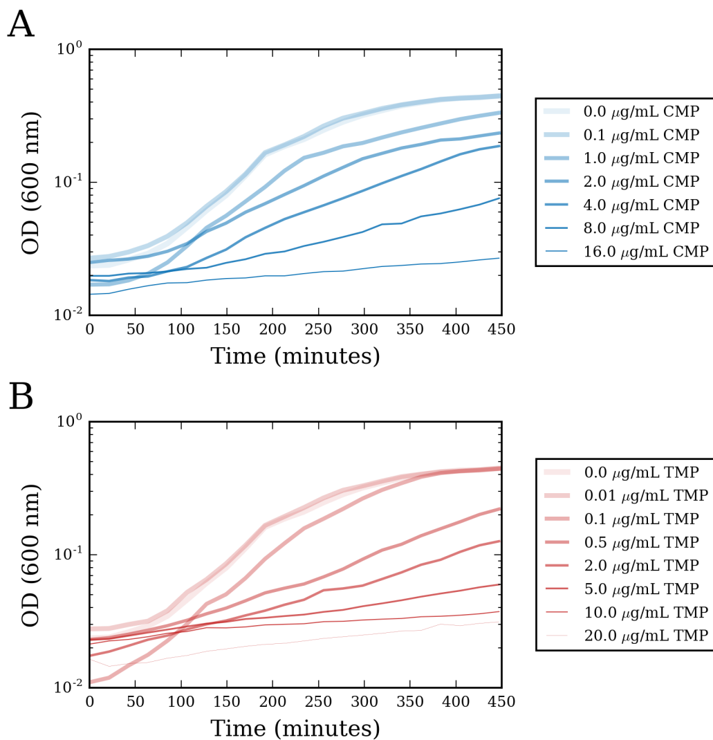
Supplementary Figure 2: Growth curves of the initial population. Growth curves of the initial barcoded population in the presence of (A) 0-16 \mu\text{g/ml} of chloramphenicol (CMP) or (B) 0-20 \mu\text{g/ml} of trimethoprim (TMP). We defined the MIC for each drug as the lowest concentration of antibiotic at which we observed no growth (see Methods ). Supplementary Table 3 contains raw growth curve data for the initial population at these different drug concentrations.
