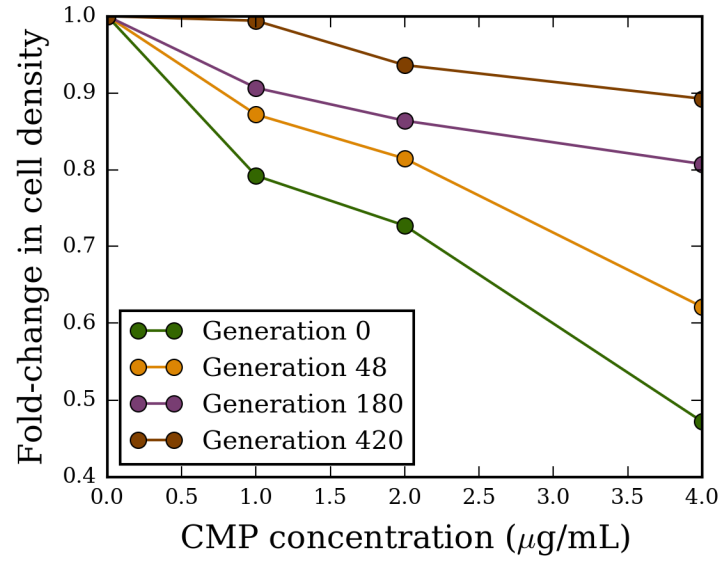
Supplementary Figure 3: Calibration of drug concentration based on population growth. Fold-change in cell density as a function of chloramphenicol (CMP) concentration for barcoded populations at four time points of the evolution experiment.
