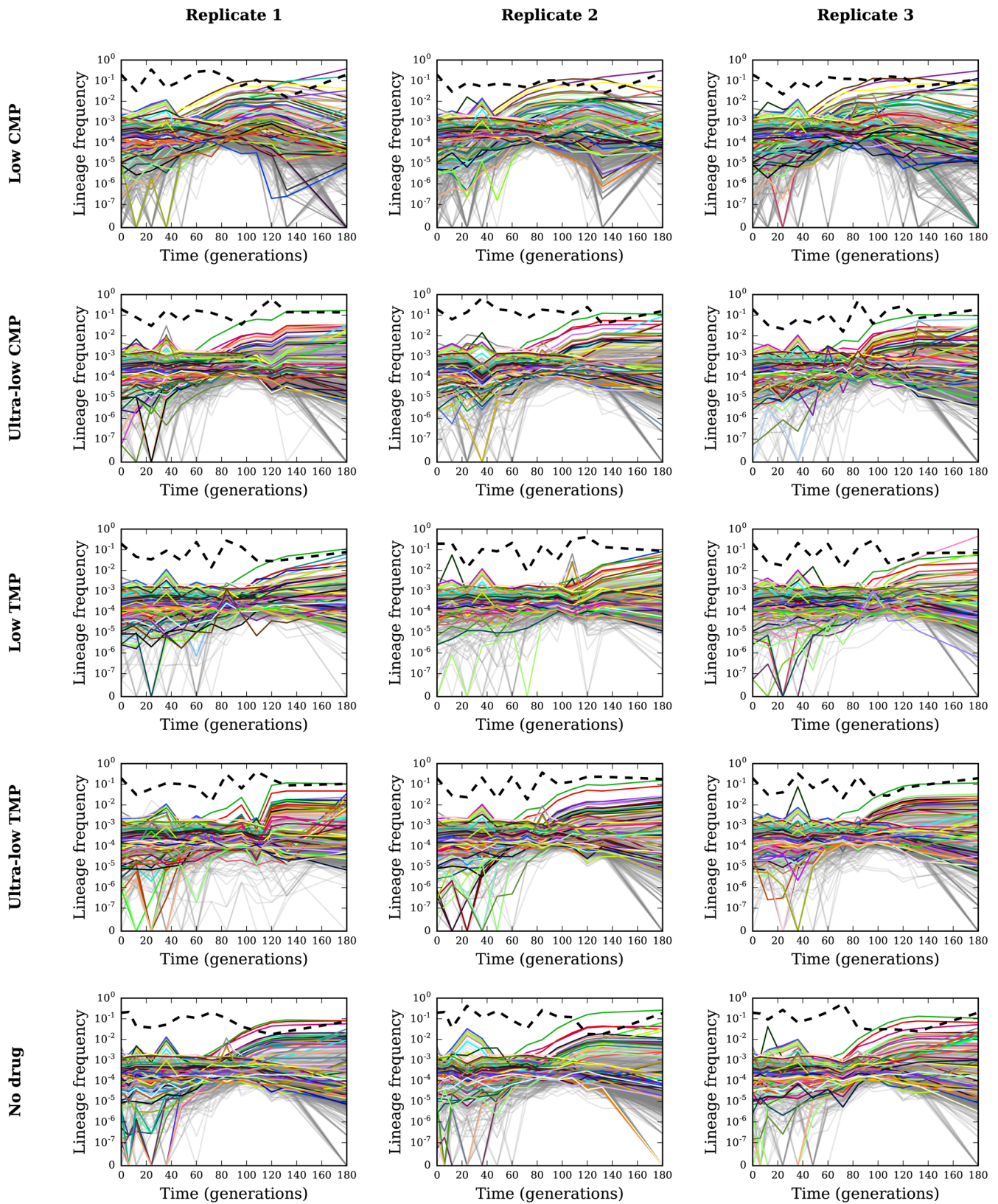
Extended Data Fig. 5 | Trajectories of barcoded lineage frequencies under constant conditions. Same as Extended Data 4 but for evolution experiments with constant drug concentrations (see Methods).
