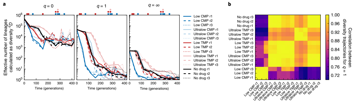
Fig. 3 | Dynamics of lineage diversity over time. a , For each population and at each time point, we measured the effective number of barcoded lineages using the diversity index {}^qD (equation (1); see also Methods) for three different values of q , which controls the weight of low- versus high-frequency lineages: {}^0D (number of unique barcodes, left), {}^1D (Shannon diversity, centre), and {}^\infty D (reciprocal of the maximum lineage frequency, right). Dots above each plot mark times at which drug concentrations changed (Extended Data Fig. 2a,b); their colours indicate the drug environment according to the key. b , Pearson correlation coefficient between diversity trajectories (for {}^1D ) from all pairs of populations. r1, replicate 1; r2, replicate 2; r3, replicate 3.
