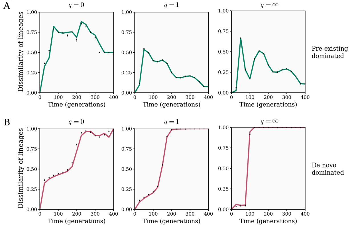
Supplementary Figure 21: Effect of subsampling on estimated dissimilarity of lineages. (A) For two simulated populations in the “pre-existing dominated” case (see Methods ), we calculated the dissimilarity of lineages ( Eq. 2 ; see also Methods ) between populations as in Extended Data Fig. 10B , but comparing both the true dissimilarity of the whole populations (solid lines) and the estimated dissimilarities based on subsampling 10% of the populations (points, with mean and standard error based on three trials). (B) Same as (A) but for simulated populations in the “de novo dominated” case (see Methods ).
