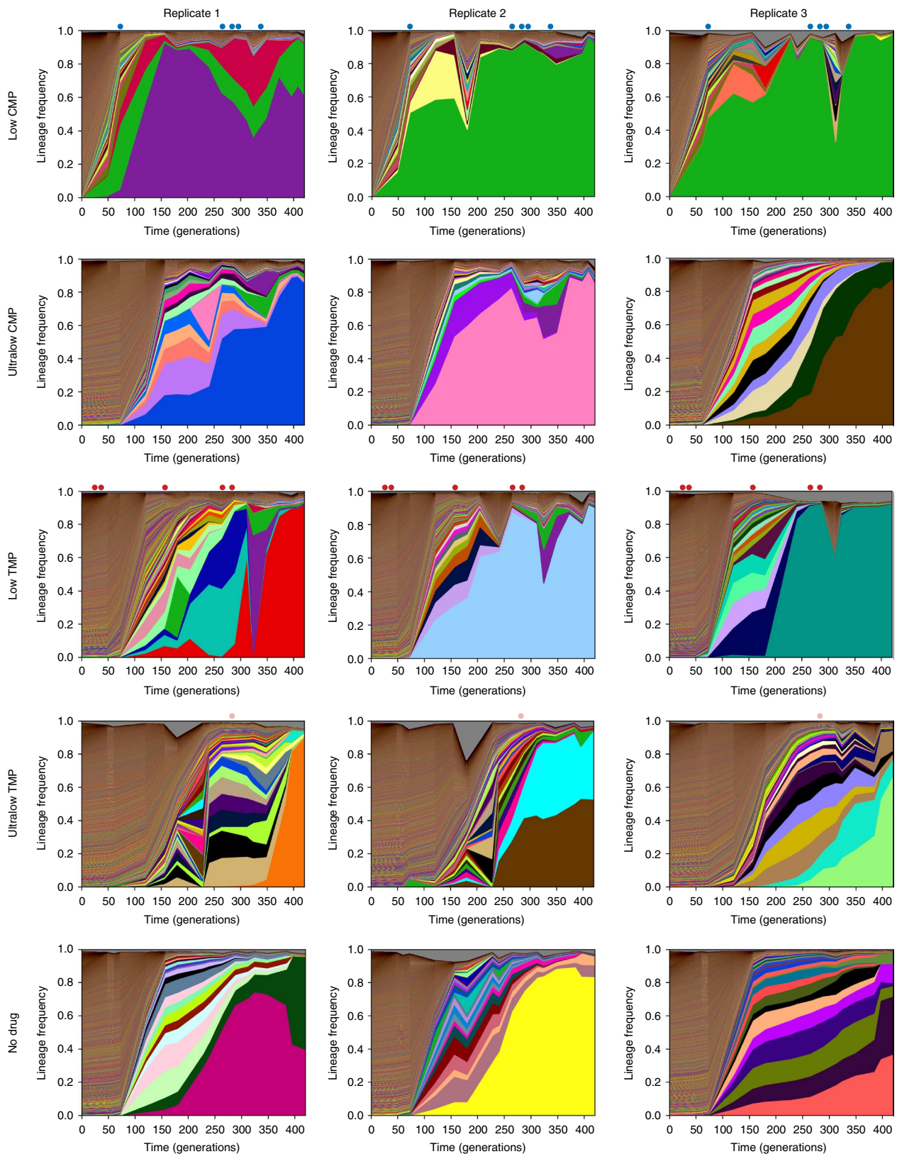
Fig. 2 | Dynamics of barcoded lineage frequencies over evolution experiment. Each row corresponds to a different antibiotic regimen, while each column corresponds to a different replicate. Individual panels show the frequency trajectories for all barcoded lineages in single populations over time of the experiment. Each coloured band corresponds to a unique lineage, with its vertical width indicating its frequency at a particular time point. For the top 20 lineages in each population (ranked by mean frequency over time), we assign a unique colour to each lineage that is consistent across panels, that is, the same colour represents the same barcode across panels (Supplementary Table 4). We use random colours for all lower-frequency lineages. The grey band at the top represents the frequency of reads without identified barcodes. Dots above each plot mark times at which the drug concentration for that population changed (Extended Data Fig. 2a,b).
