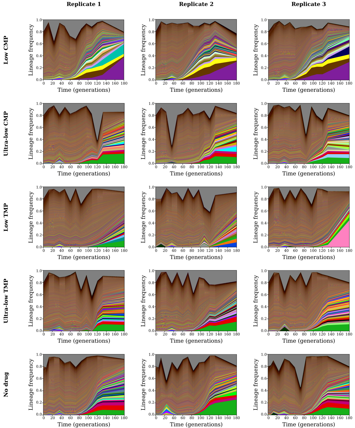
Supplementary Figure 16: Dynamics of barcoded lineage frequencies over evolution experiment under constant conditions. Same as Fig. 2 but for evolution experiments with constant drug concentrations (see Methods).
