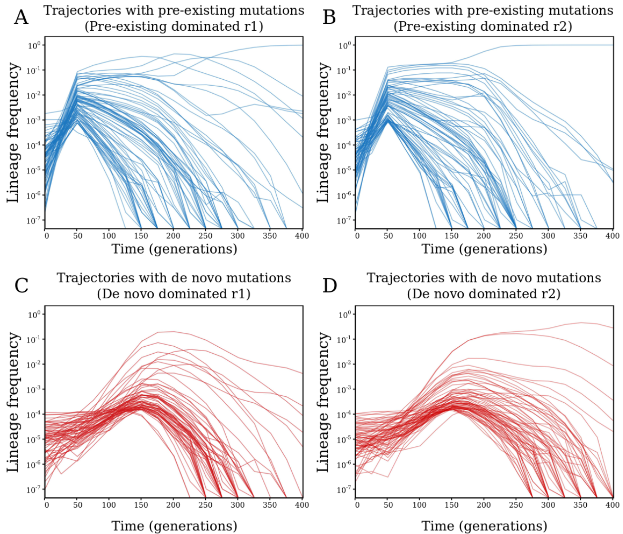
Supplementary Figure 19: Simulated trajectories from pre-existing versus de novo mutations. (A, B) For two simulated populations in the “pre-existing dominated” case (see Methods ), we show barcoded lineage trajectories with pre-existing beneficial mutations. (C, D) For two simulated populations in the “de novo dominated” case (see Methods ), we show barcoded lineage trajectories that acquire beneficial mutations de novo. For simplicity, we show the lineages that rise to a minimum frequency of 10^{-4} .
