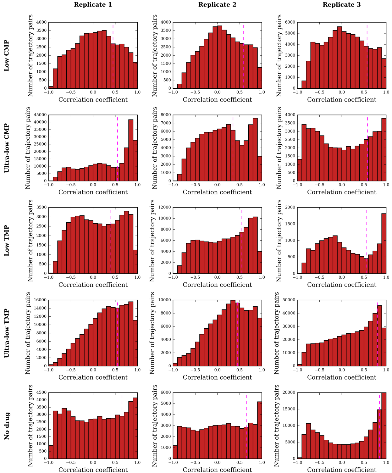
Supplementary Figure 12: Distributions of trajectory correlations. Each row corresponds to a different antibiotic regimen, while each column corresponds to a different replicate. Individual panels show histograms of Pearson correlation coefficients between all pairs of lineage trajectories used for hierarchical clustering in each population (see Methods ). The vertical dashed lines mark the thresholds for forming flat clusters.
