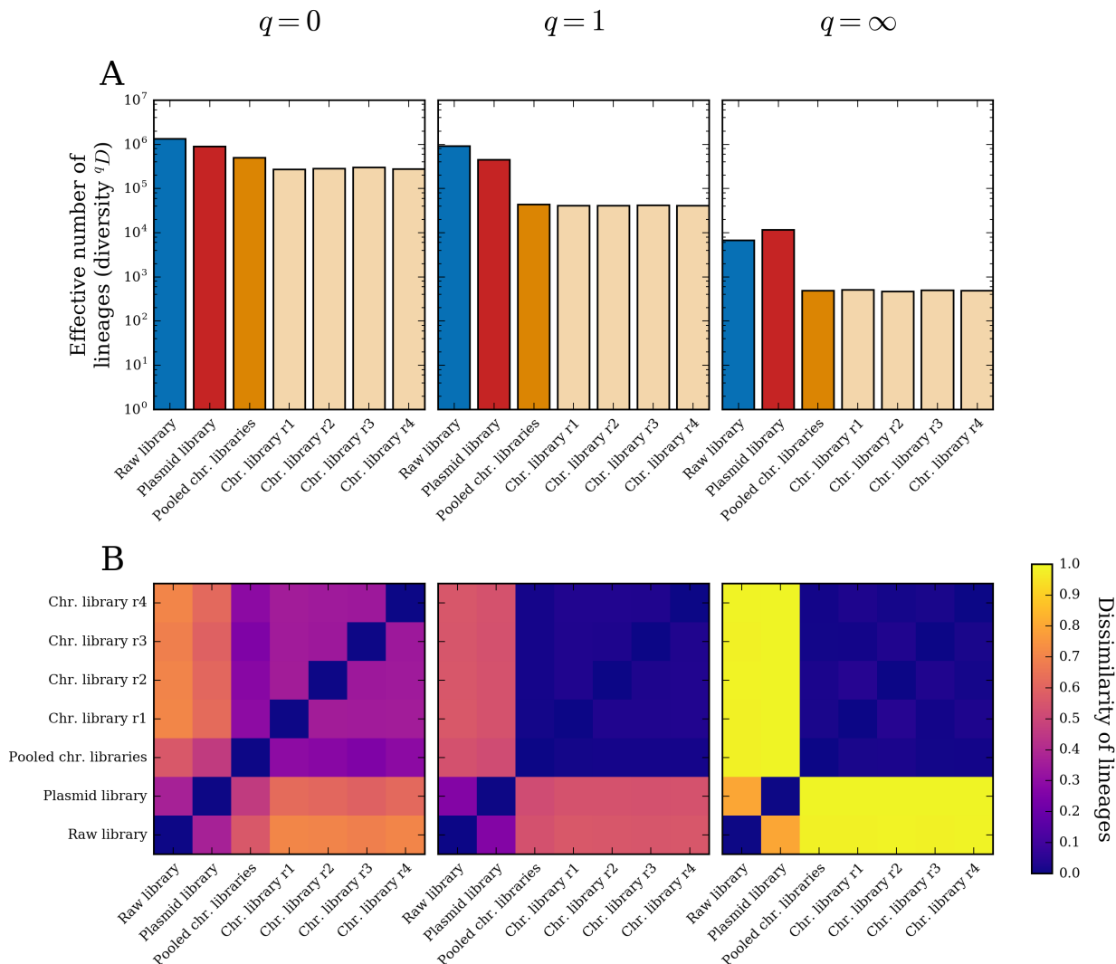
Supplementary Figure 5: Lineage diversity within and between initial libraries. (A) For each initial barcode library (same as in Extended Data Fig. 1 , except with the four independent samples of the chromosomal library shown both separate and pooled), we calculate the effective number of barcoded lineages using the diversity index {}^qD ( Eq. 1 ; see also Methods ) for three different values q , which controls the weight of low- versus high-frequency lineages: {}^0D (number of unique barcodes, left), {}^1D (Shannon diversity, center), and {}^\infty D (reciprocal of the maximum lineage frequency, right). (B) Dissimilarity of lineages ( Eq. 2 ; see also Methods ) between all pairs of initial libraries from (A). Columns are the same as in (A): left, q = 0 ; center, q = 1 ; and right, q = \infty .
