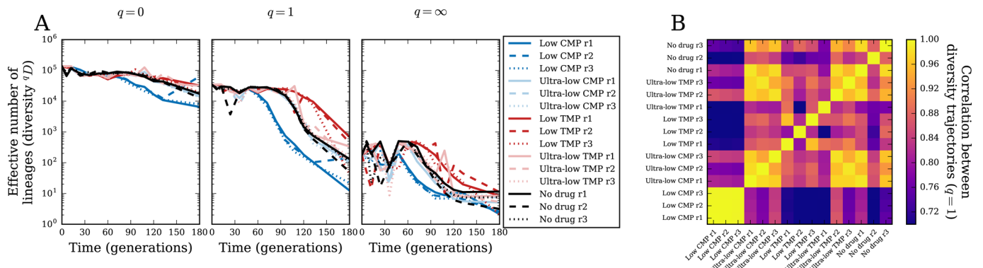
Extended Data Fig. 6 | Dynamics of lineage diversity over time under constant conditions. Same as Fig. 3 but for evolution experiments with constant drug concentrations (see Methods).
