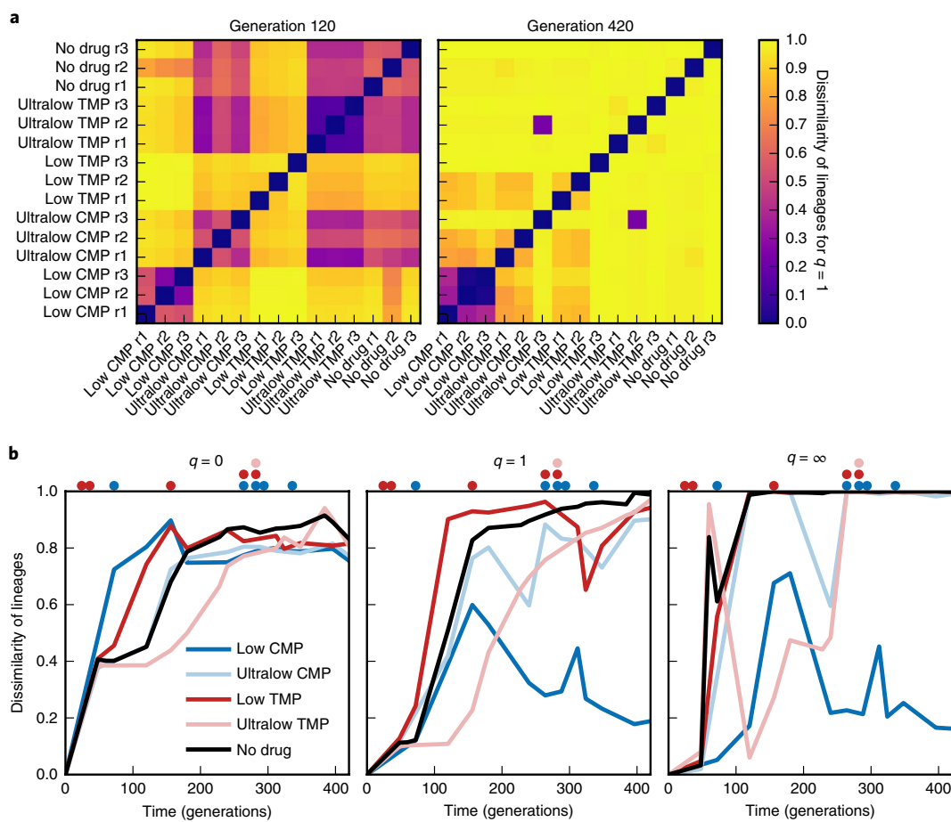
Fig. 4 | Dynamics of lineage dissimilarity among populations over time. a , Dissimilarity of lineages for q = 1 (equation (2); see also Methods) between all pairs of populations at generation 120 (left) and the final time point at generation 420 (right). b , Dissimilarity of lineages among all replicate populations in each drug condition, using q = 0 (left), q = 1 (centre) and q = \infty (right). Dots above each plot mark times at which the drug concentrations changed (Extended Data Fig. 2a,b); their colours indicate the drug environment according to the key.
