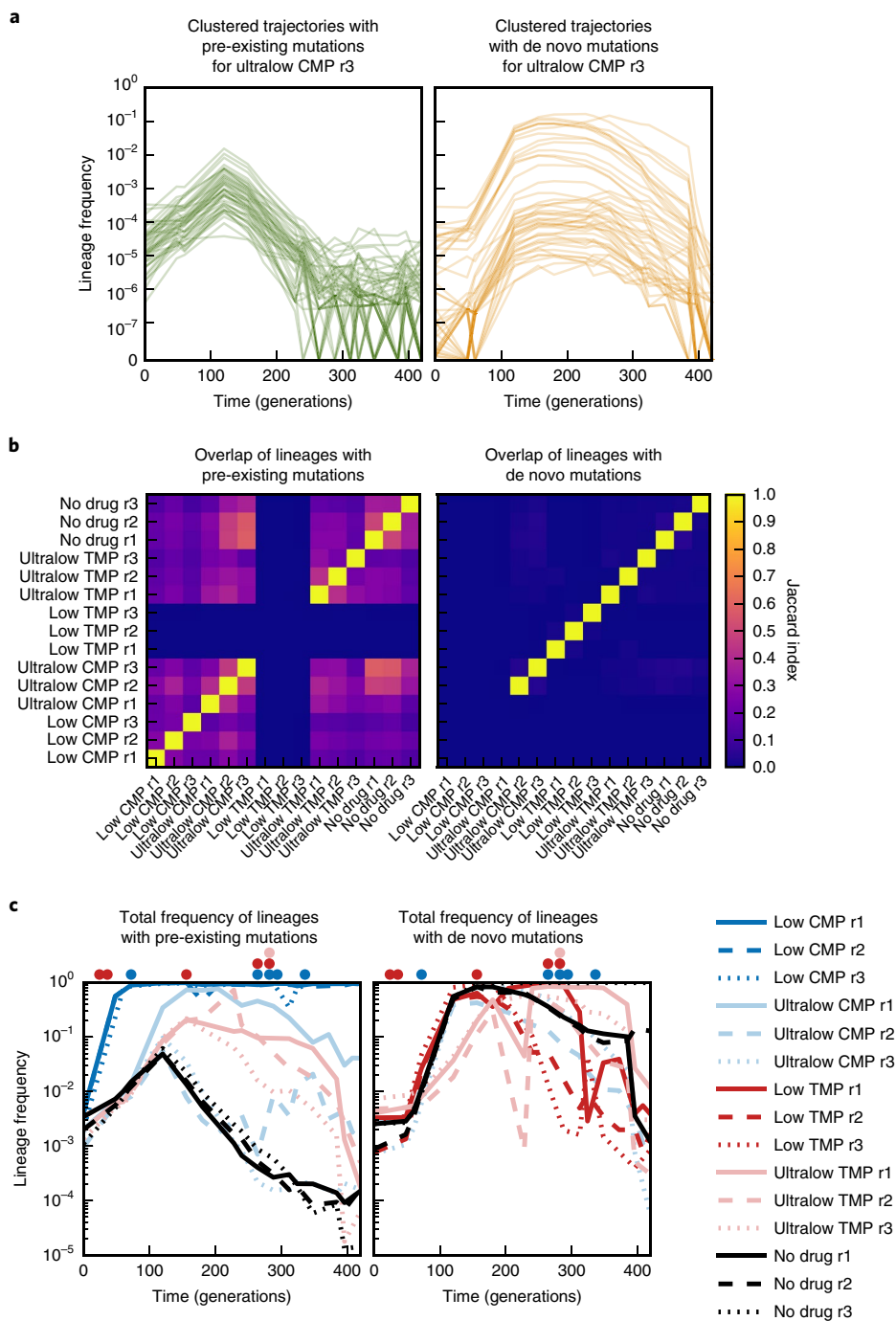
Fig. 6 | Distinct patterns of trajectories from pre-existing and de novo beneficial mutations. a , Examples of clustered lineage trajectories suggesting the presence of pre-existing beneficial mutations (left) and de novo beneficial mutations (right) from ultralow CMP replicate 3. Trajectories are partially transparent to show overlap. b , For each pair of populations, we calculated the relative overlap of lineages in trajectory clusters with apparent pre-existing beneficial mutations (left) and in clusters with apparent de novo beneficial mutations (right) (see Supplementary Fig. 13 for classification of trajectory clusters). We measured overlap using the Jaccard index, that is, the ratio of the number of lineages in the intersection to the number in the union. All entries are zero for pre-existing mutations under low TMP and for de novo mutations under low CMP because we identify no clusters of these types in those populations (Supplementary Fig. 13). c , Total frequency trajectories of all lineages with apparent pre-existing mutations (left) and with apparent de novo mutations (right) in each population. Dots above each plot mark times at which the drug concentrations changed (Extended Data Fig. 2a, b); their colours indicate the drug environment according to the key.
