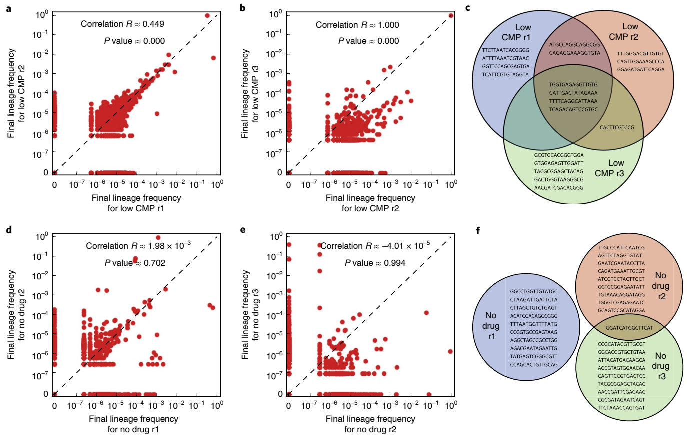
Fig. 5 | Reproducibility of individual lineage dynamics. a, b , Comparison of final frequencies of all barcoded lineages under low CMP conditions between replicate populations 1 and 2 ( a ) and between replicate populations 2 and 3 ( b ). The dashed black line marks the line of identity; each panel also shows the Pearson correlation coefficient R and estimated P value for the frequencies ( P values are numerically indistinguishable from zero). c , Venn diagram of the top ten barcodes (ranked by mean frequency over time) in each replicate population from low CMP. d–f , Same as a–c but for three replicate populations without drug.
