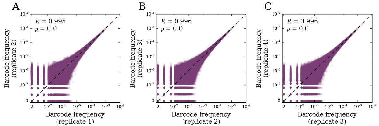
Supplementary Figure 1: Reproducibility of barcode frequency measurements. We compared measured barcode frequencies between four independent sequencing runs on the initial chromosomal library: (A) replicates 1 and 2, (B) replicates 2 and 3, and (C) replicates 3 and 4. Points are partially transparent to show their density; the dashed black line marks the line of identity. We also show the Pearson correlation coefficient R and estimated p -value for the frequencies ( p -values are numerically indistinguishable from zero).
