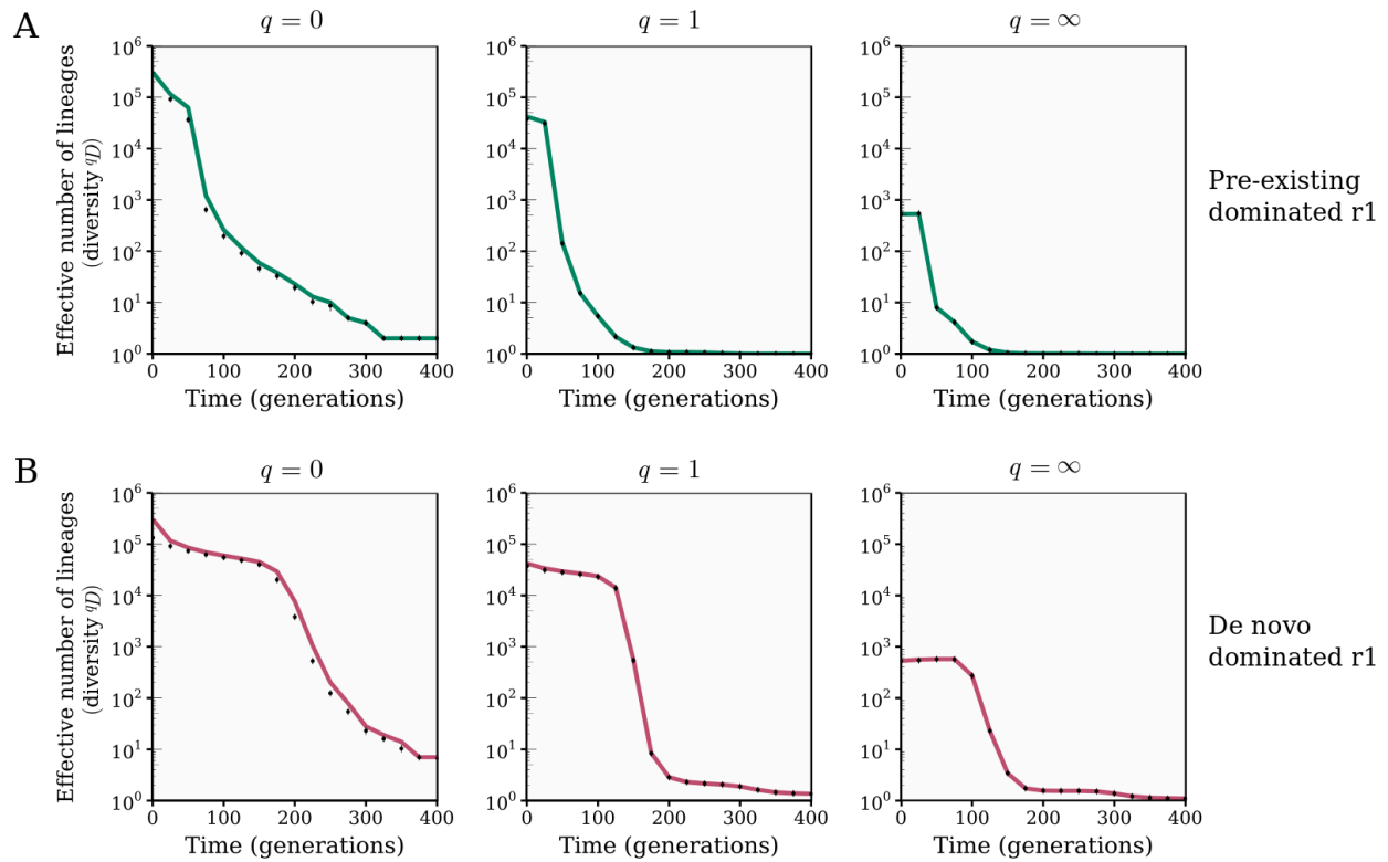
Supplementary Figure 20: Effect of subsampling on estimated diversity. (A) For a simulated population in the “pre-existing dominated” case (see Methods ), we calculated the effective number of barcoded lineages using the diversity index {}^qD (Eq. 1; see also Methods ) as in Extended Data Fig. 10A , but comparing both the true diversity of the whole population (solid lines) and the estimated diversity based on subsampling 10% of the population (points, with mean and standard error based on three trials). (B) Same as (A) but for a simulated population in the “de novo dominated” case (see Methods ).
