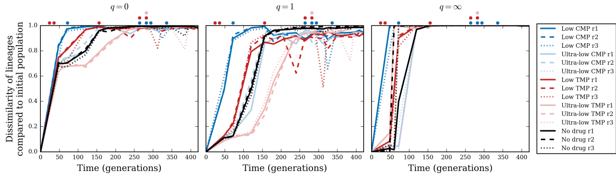
Supplementary Figure 10: Divergence of lineage dissimilarity over evolution. For each population at each time point, we calculate the dissimilarity of lineages (Eq. 2; see also Methods ) with the initial population for q = 0 (left), q = 1 (center), and q = \infty (right). Dots above each plot mark times at which the drug concentrations changed ( Extended Data Fig. 2A,B ).
